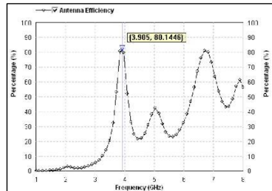
Fig 8: Radiation Efficiency Vs Frequency Curve
