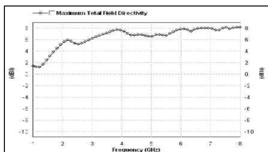
Fig 6: Directivity Vs Frequency Curve
