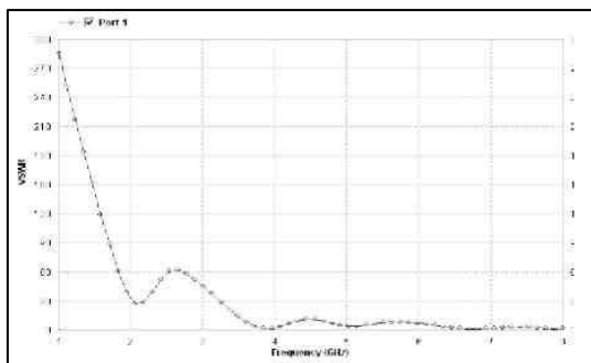
Fig 4: VSWR Vs Frequency Curve
