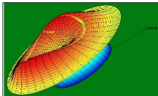
Fig 9: 3d Radiation Pattern of Back to Back E Shape Antenna
